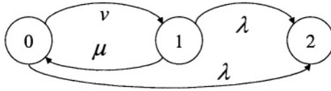
Fig. 3.4. Markov model considering intermittent faults.
