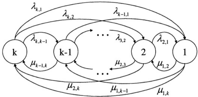
Fig. 8.5. CTMC for general repairable MSS element.
