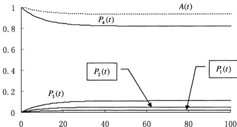
Fig. 8.6. State probabilities of the repairable 4-state system.
